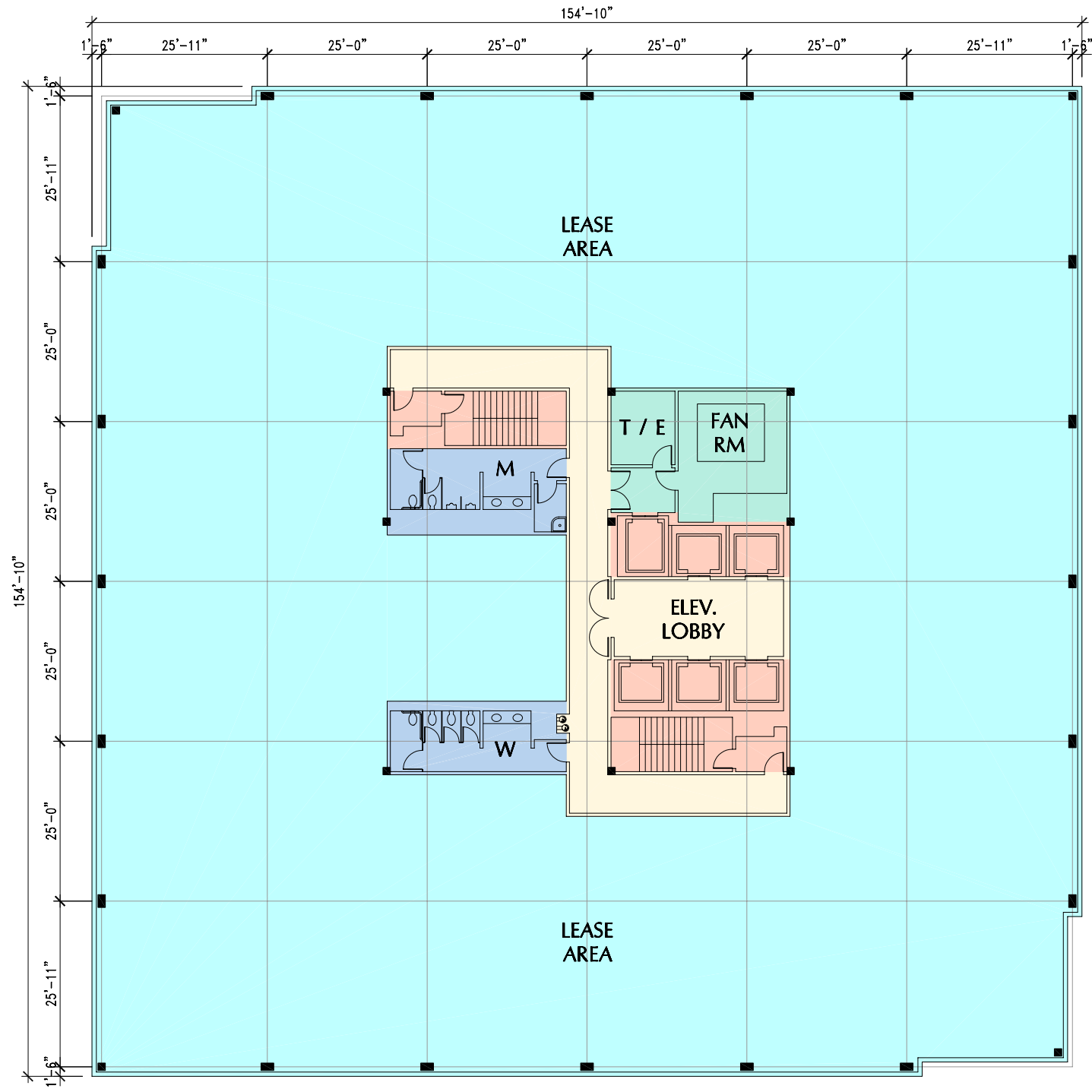
TYPICAL FLOOR
